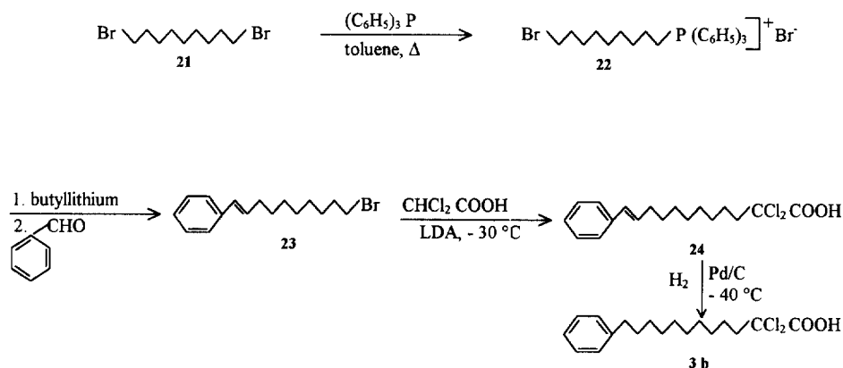
Figure 4. Synthesis of 2,2-dichloro-12-phenyl-11-dodecenoic acid and 2,2-dichloro-12-phenyl-dodecanoic acid.
