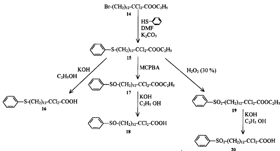
Figure 3. Synthesis of sulphur-containing 2,2-dichlorocarboxylic acids.
